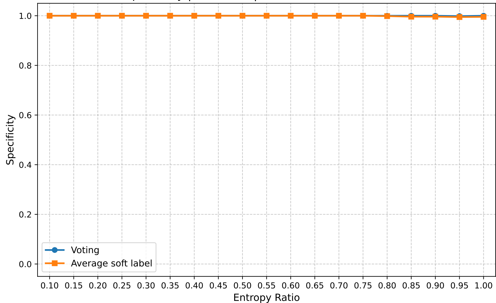
Specificity | Round 20 | Confuse Model Ratio 0.30
