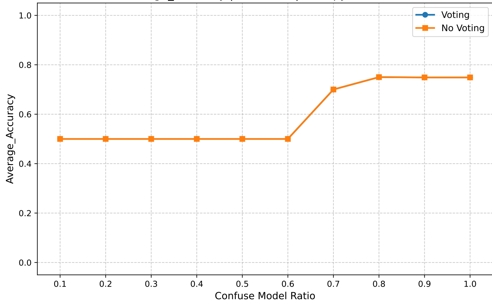
Average_Accuracy | Round 10 | Entropy Ratio 0.10
