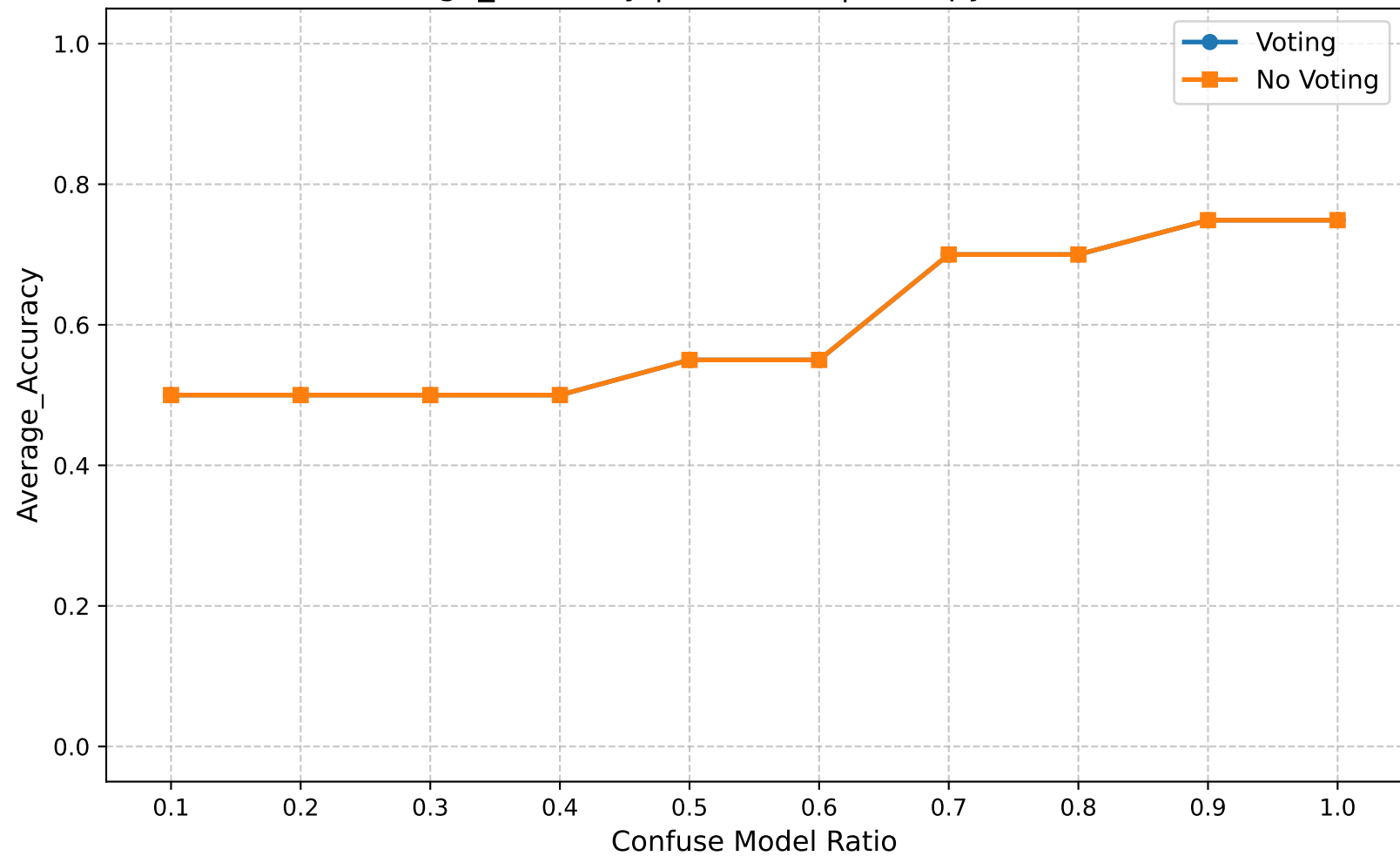
Average_Accuracy | Round 15 | Entropy Ratio 0.15
