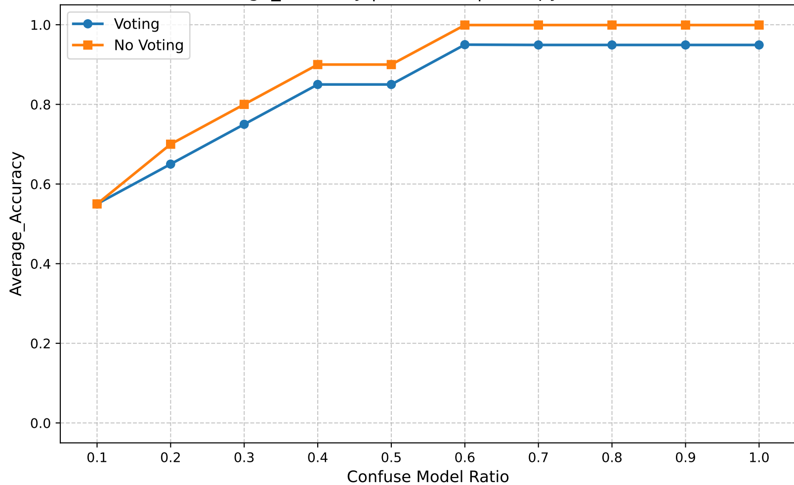
Average_Accuracy | Round 15 | Entropy Ratio 0.40
