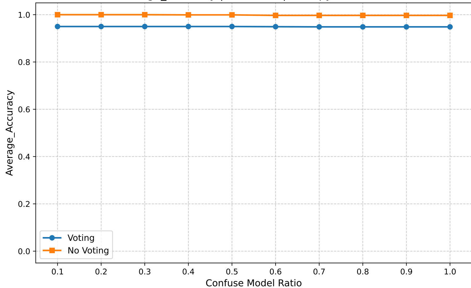
Average_Accuracy | Round 15 | Entropy Ratio 0.80
