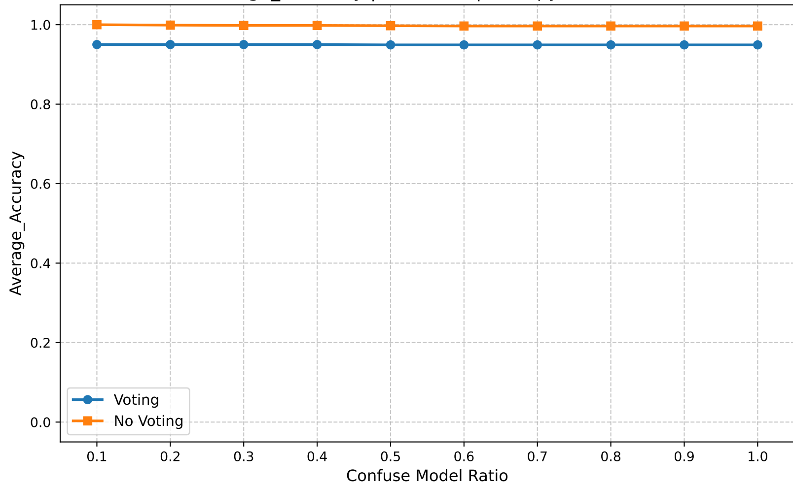
Average_Accuracy | Round 15 | Entropy Ratio 0.85
