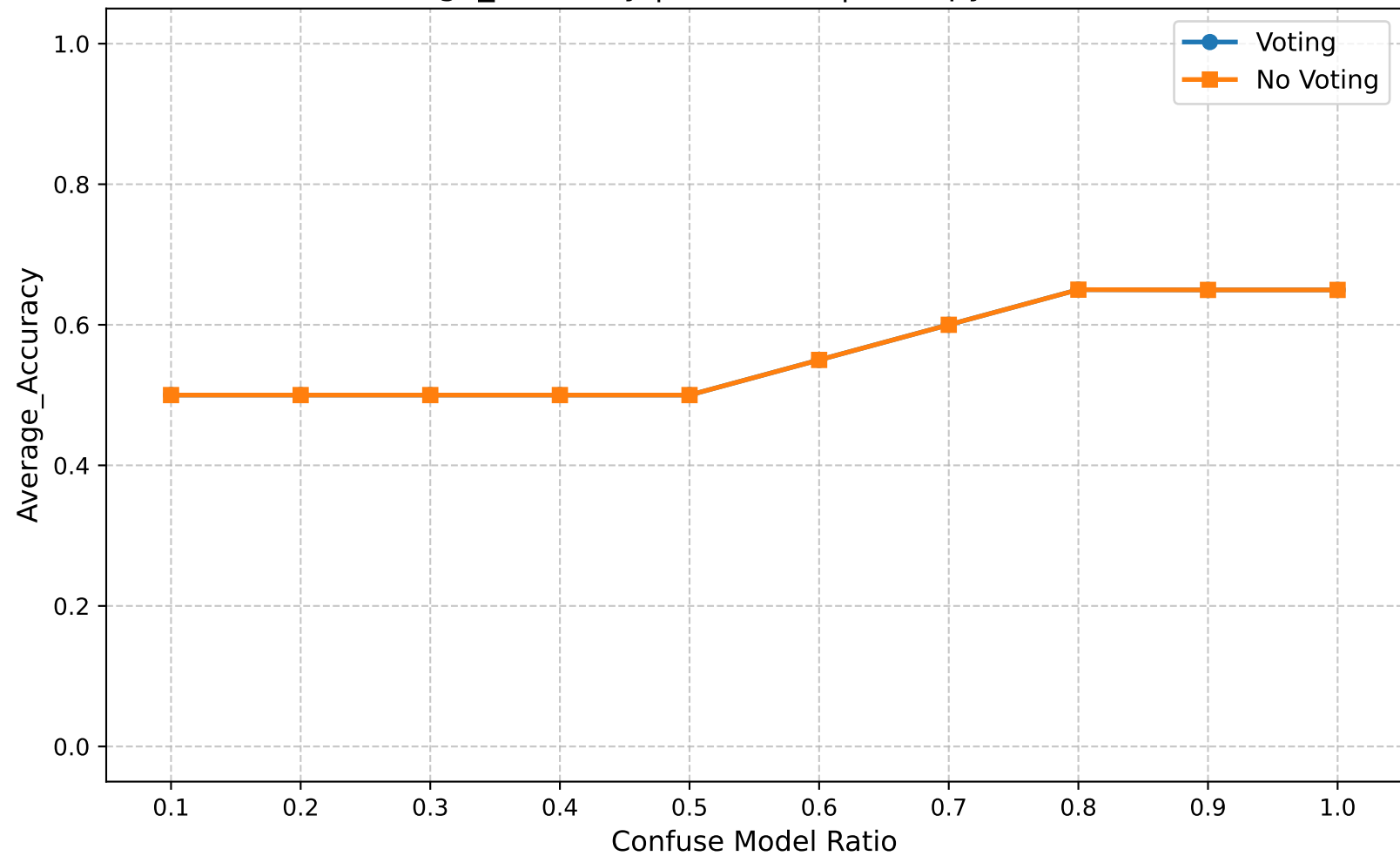
Average_Accuracy | Round 20 | Entropy Ratio 0.10
