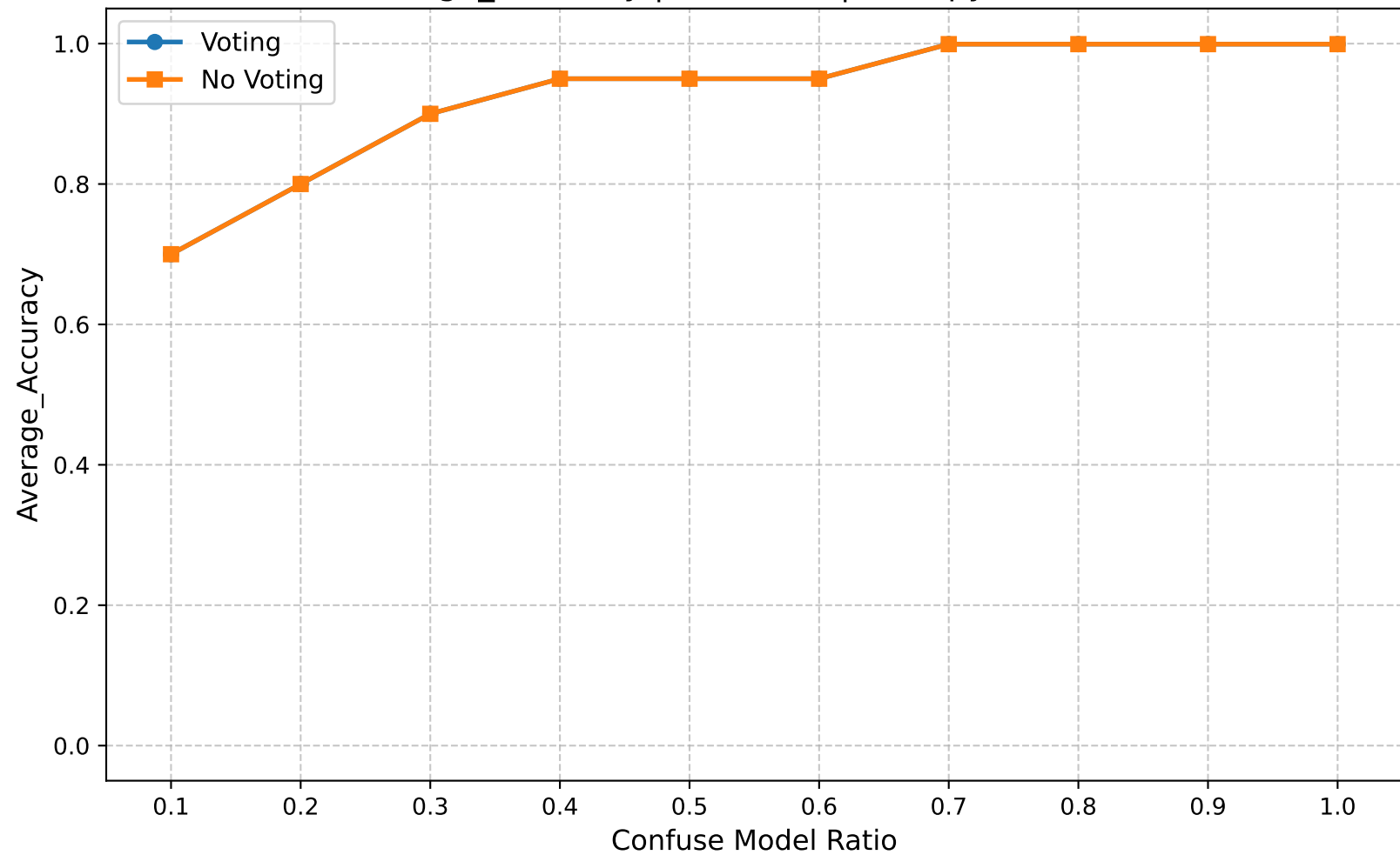
Average_Accuracy | Round 20 | Entropy Ratio 0.45
