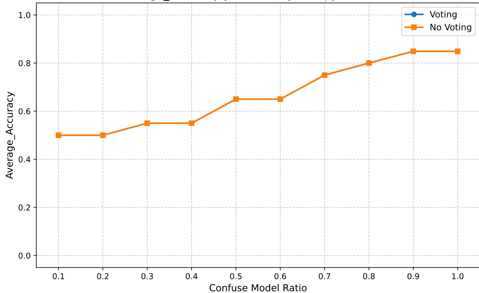
Average_Accuracy | Round 25 | Entropy Ratio 0.20
