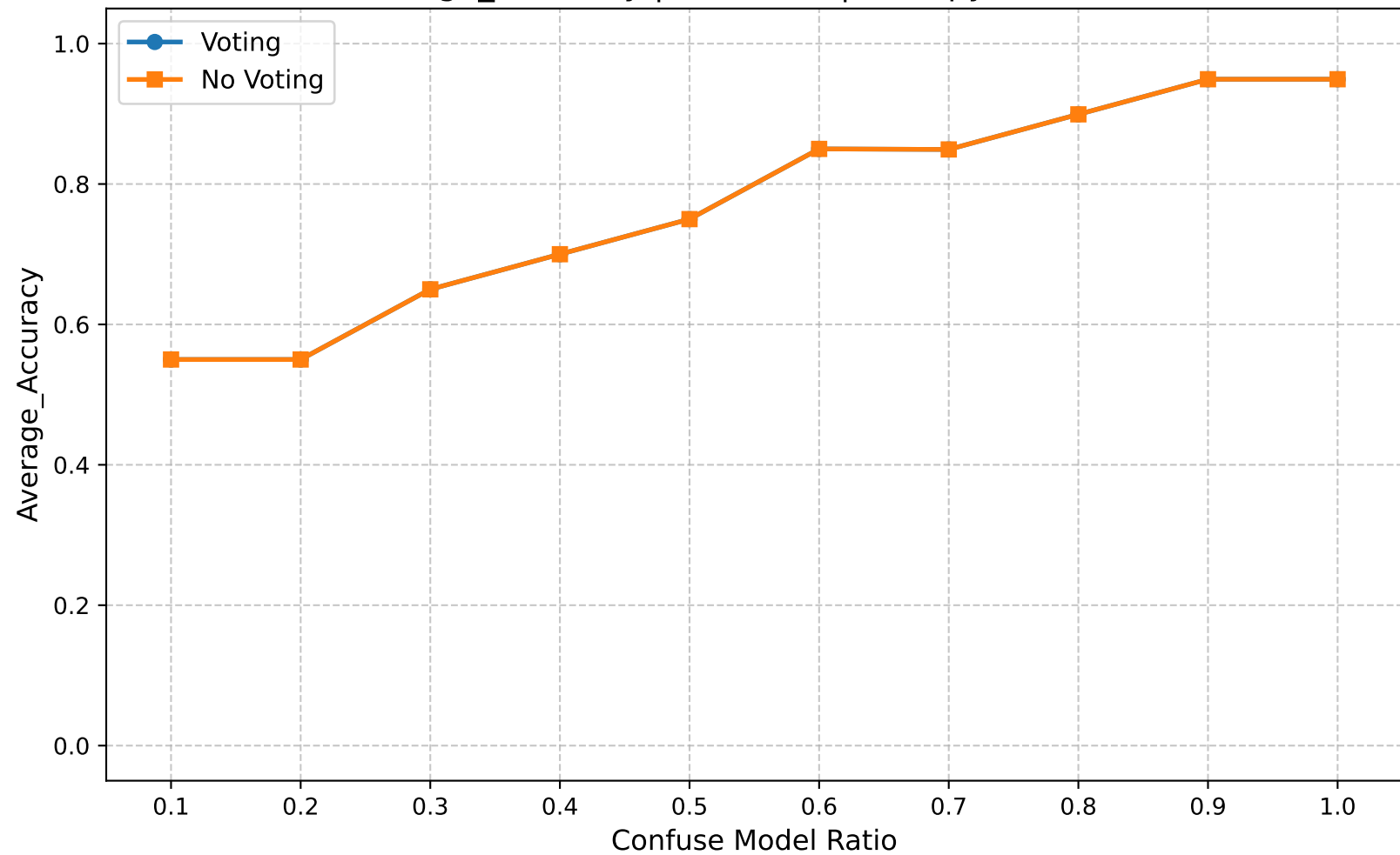
Average_Accuracy | Round 25 | Entropy Ratio 0.30
