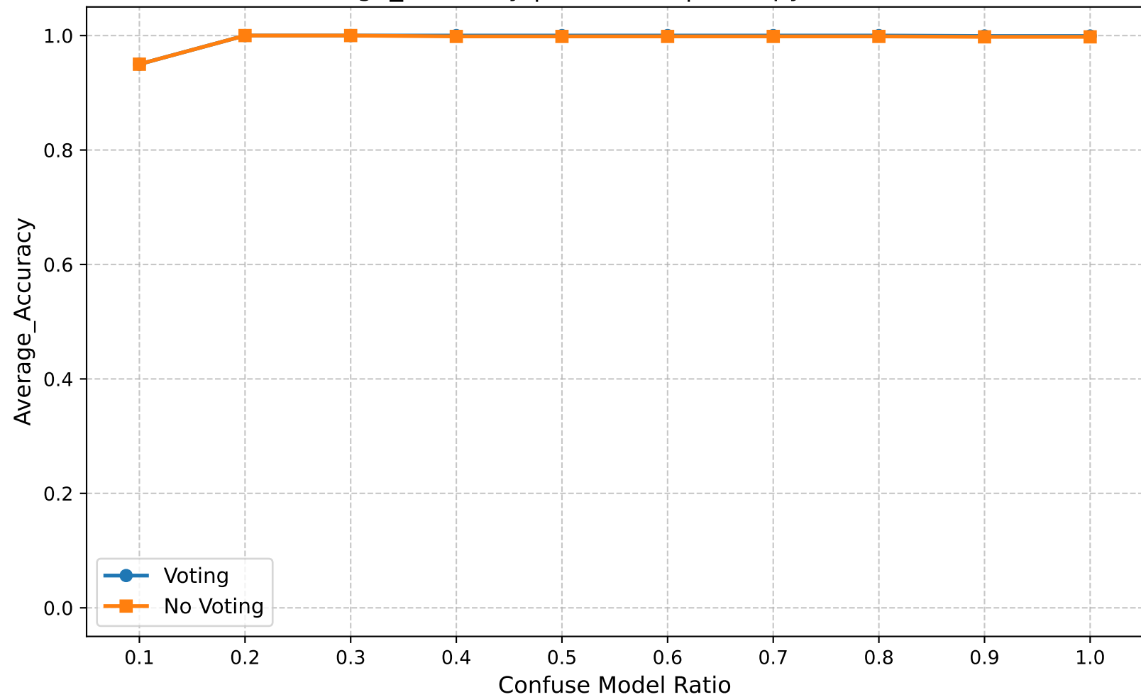
Average_Accuracy | Round 25 | Entropy Ratio 0.65
