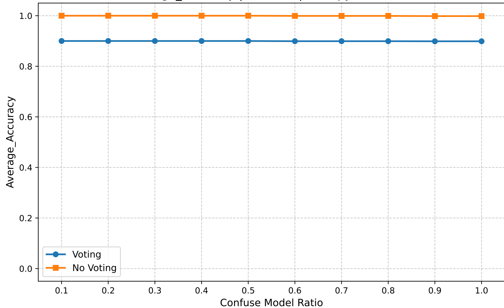
Average_Accuracy | Round 5 | Entropy Ratio 0.70
