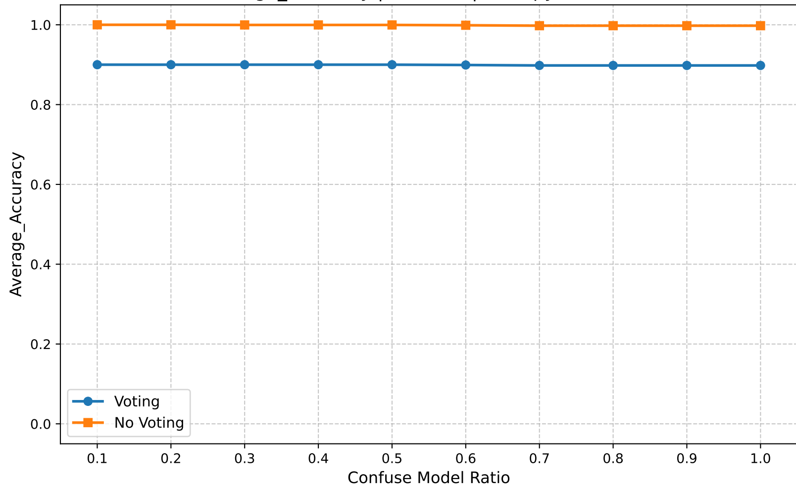
Average_Accuracy | Round 5 | Entropy Ratio 0.80
