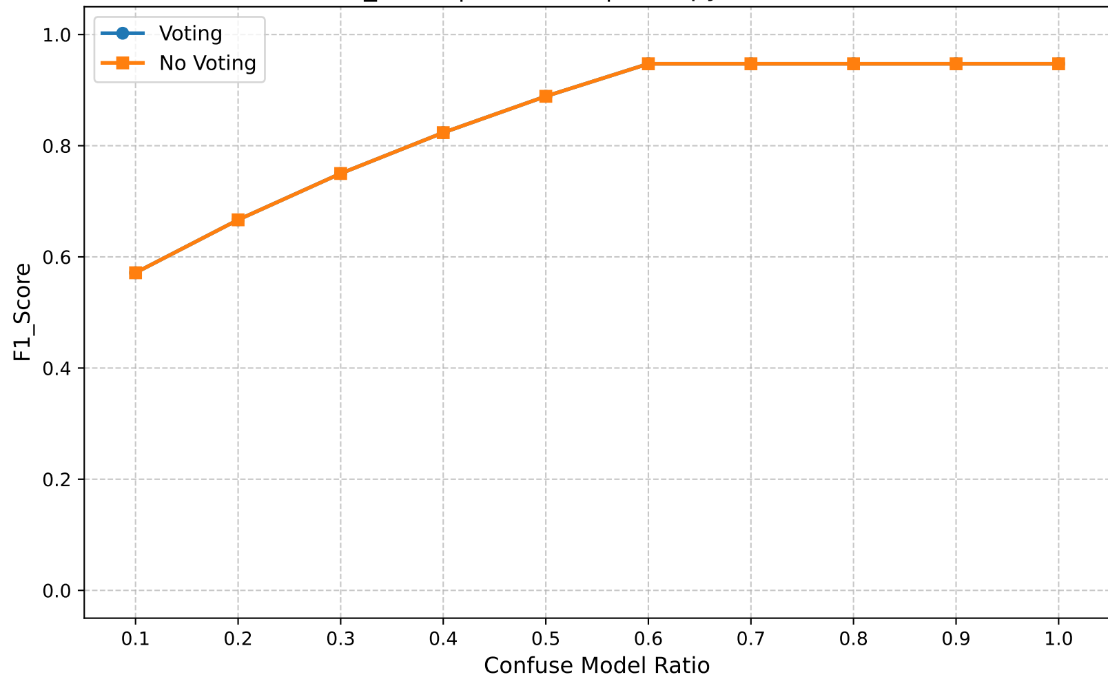
F1_Score | Round 10 | Entropy Ratio 0.45
