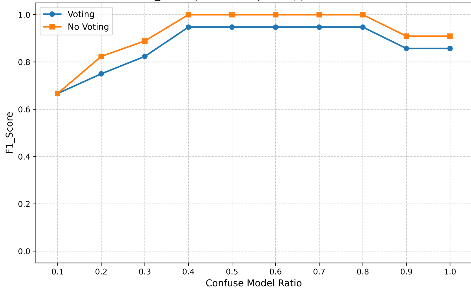
F1_Score | Round 10 | Entropy Ratio 0.55
