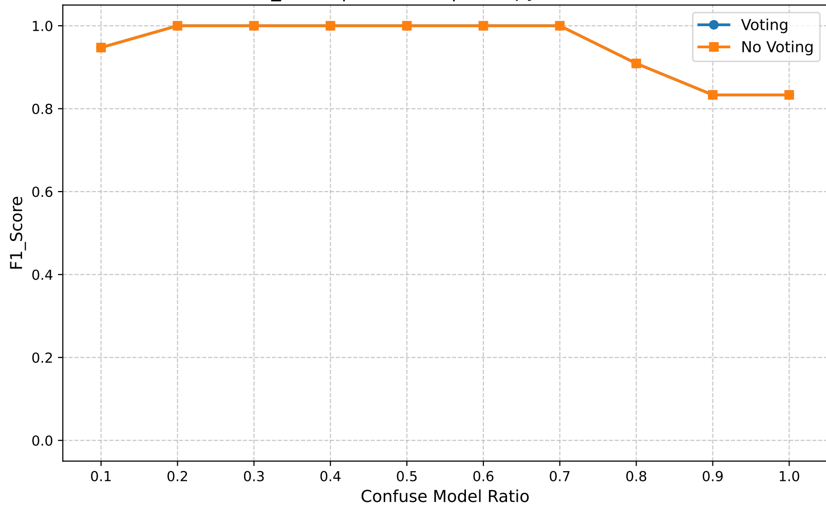
F1_Score | Round 10 | Entropy Ratio 0.65
