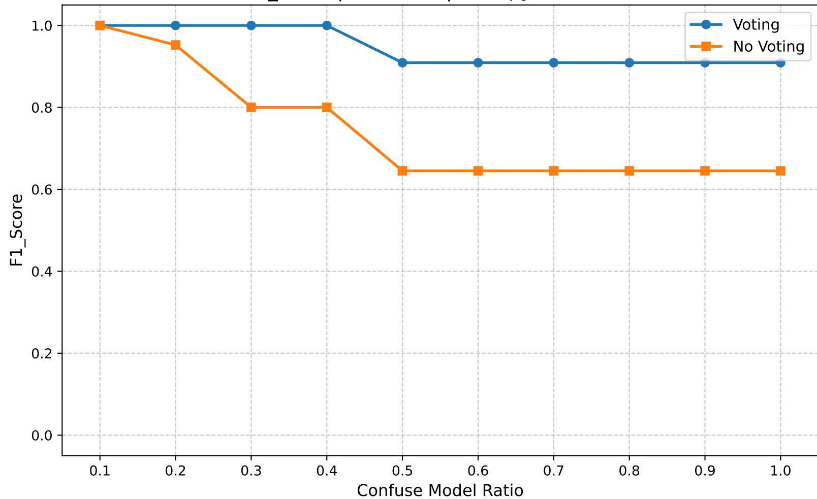
F1_Score | Round 10 | Entropy Ratio 0.85
