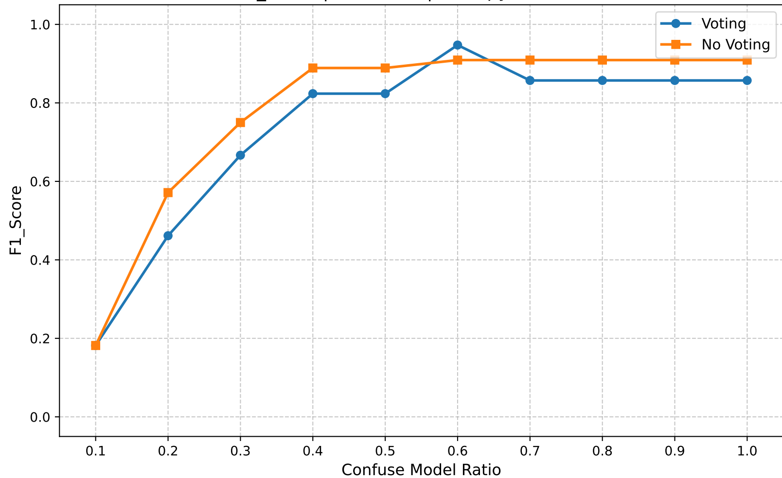
F1_Score | Round 15 | Entropy Ratio 0.40
