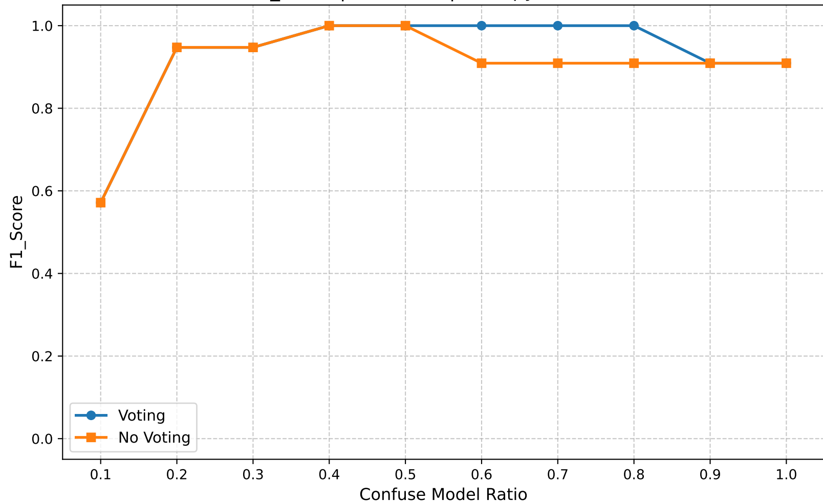
F1_Score | Round 15 | Entropy Ratio 0.50
