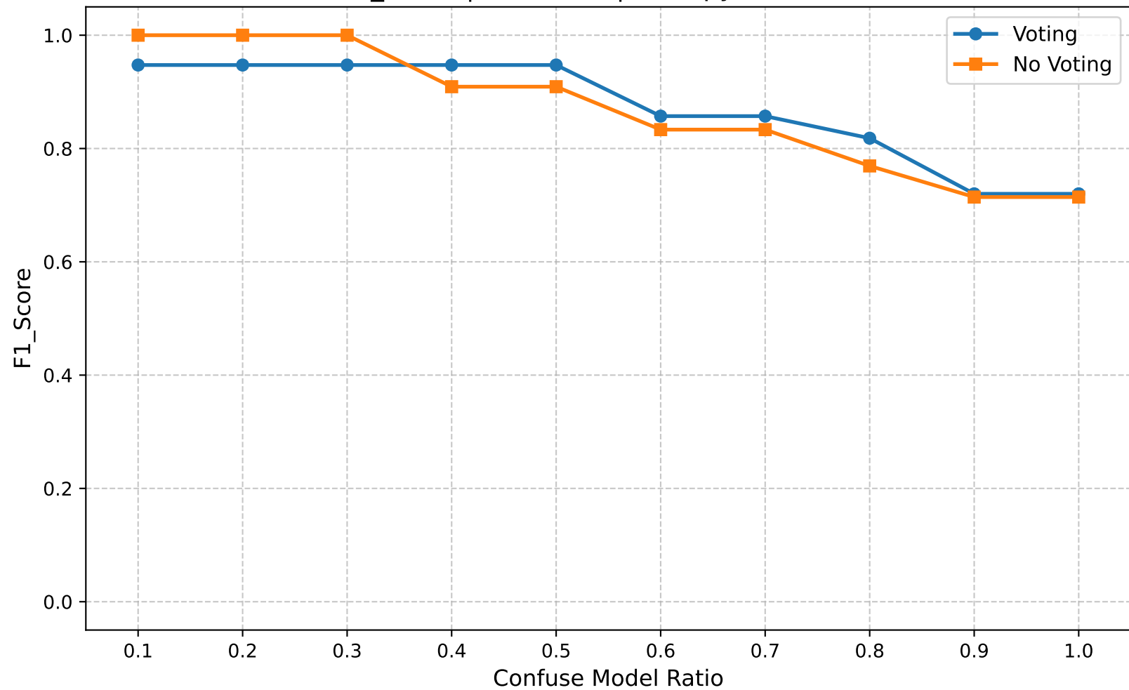
F1_Score | Round 15 | Entropy Ratio 0.75
