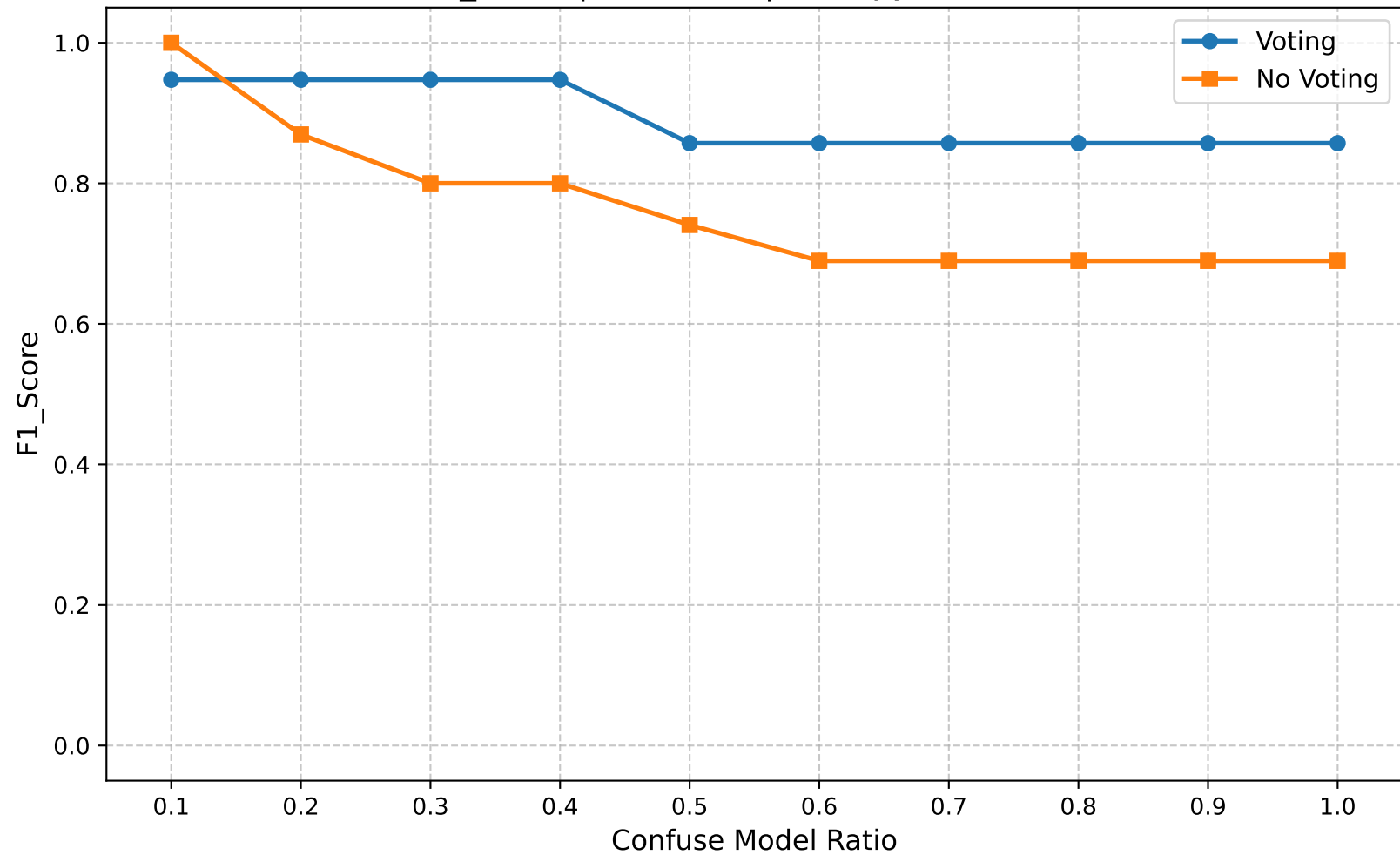
F1_Score | Round 15 | Entropy Ratio 0.85
