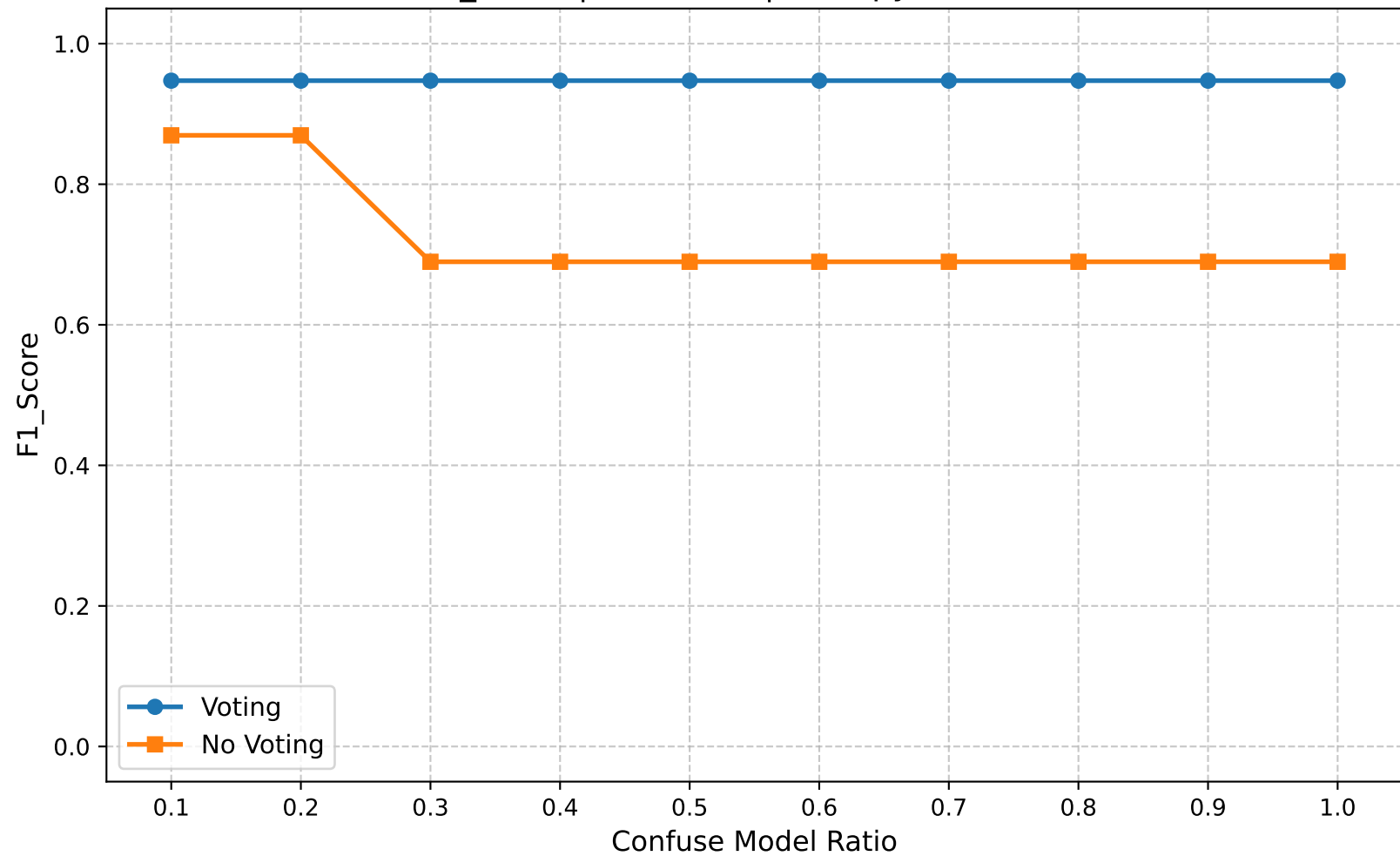
F1_Score | Round 15 | Entropy Ratio 0.95
