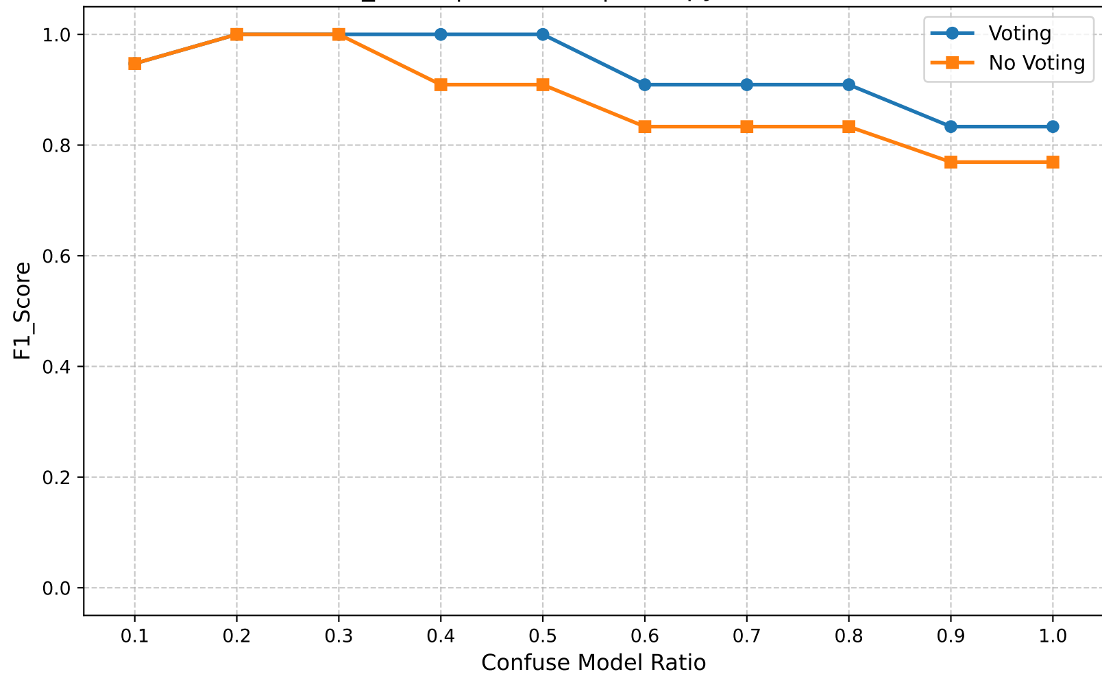
F1_Score | Round 20 | Entropy Ratio 0.75
