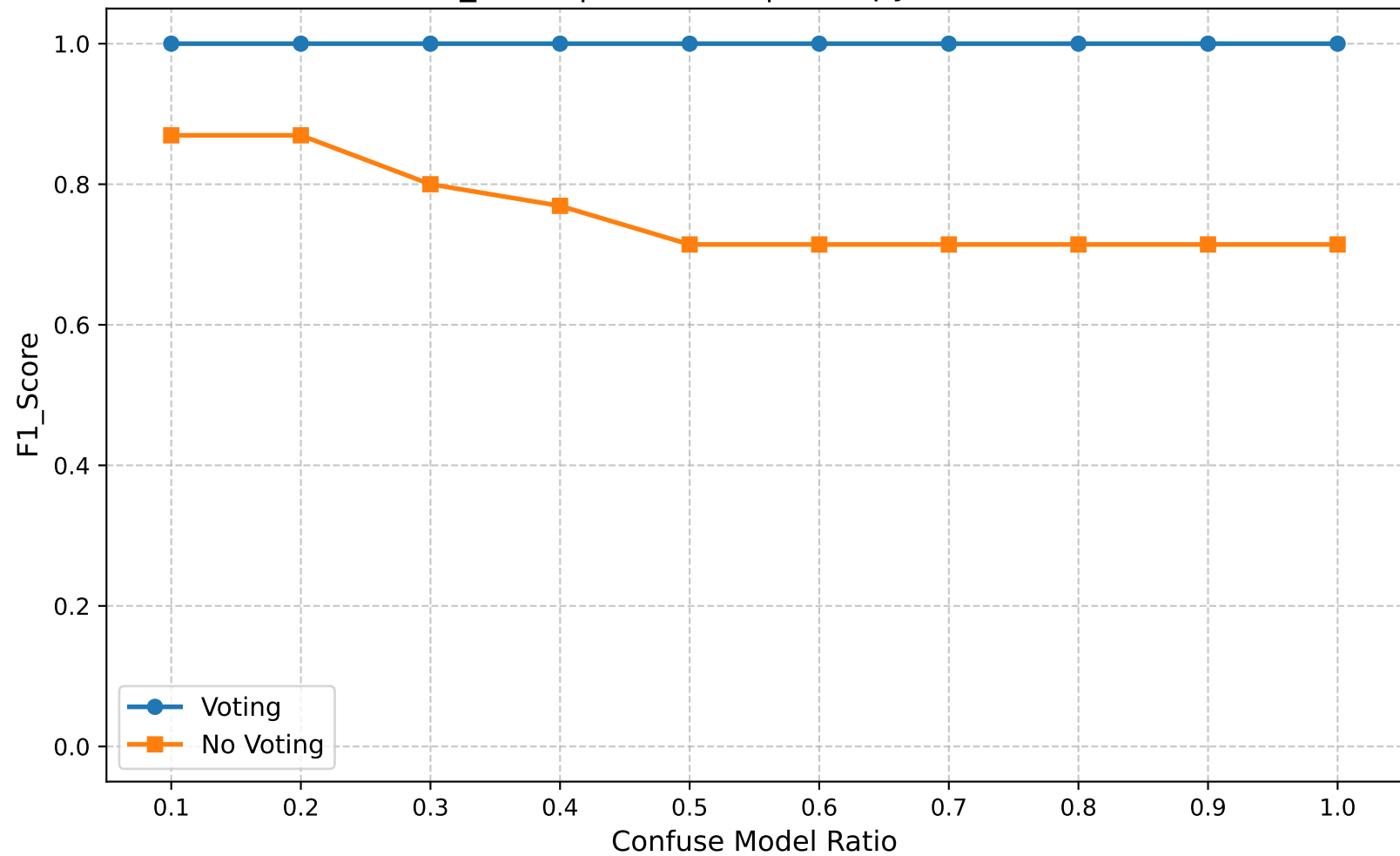
F1_Score | Round 20 | Entropy Ratio 0.90
