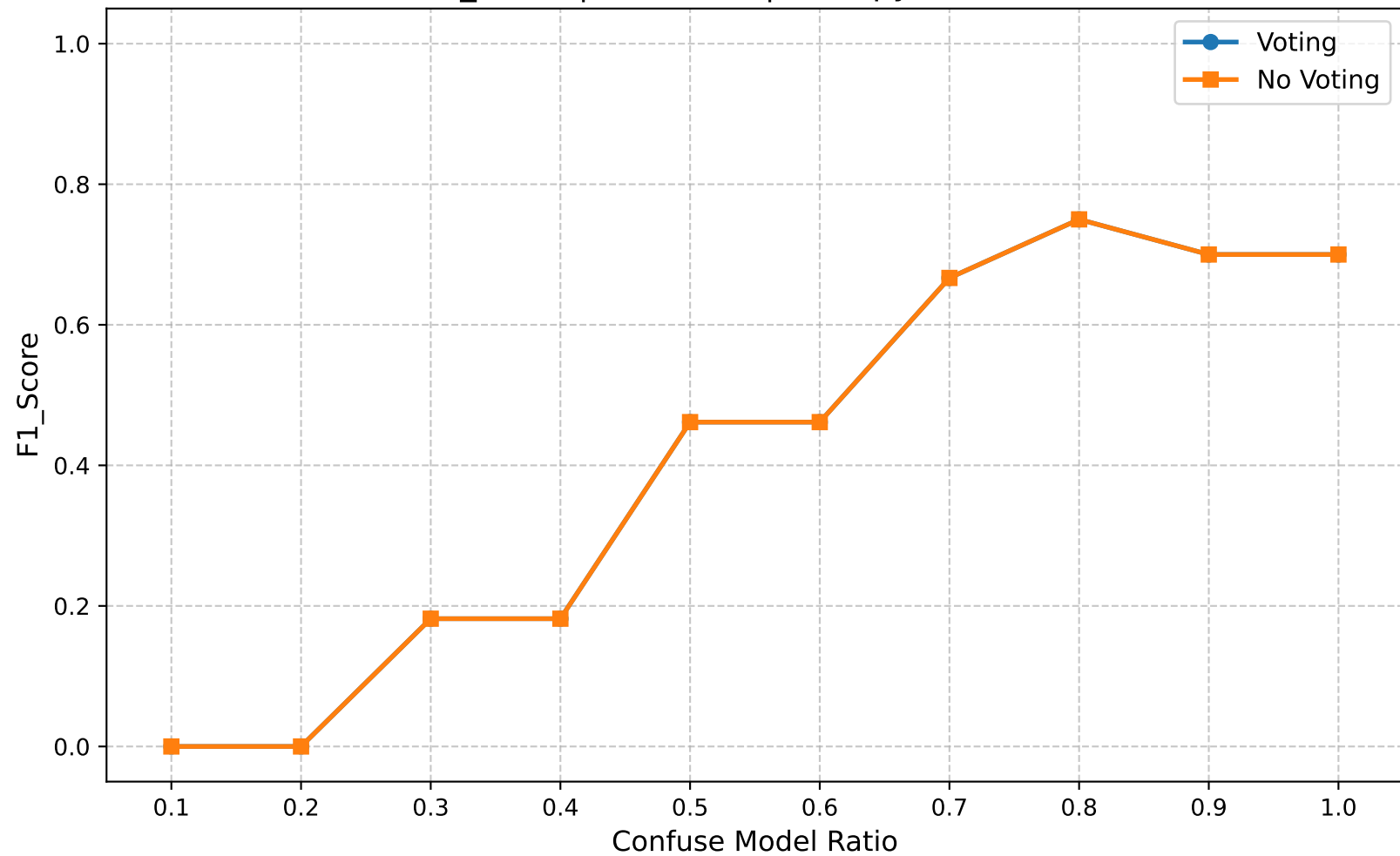
F1_Score | Round 25 | Entropy Ratio 0.20
