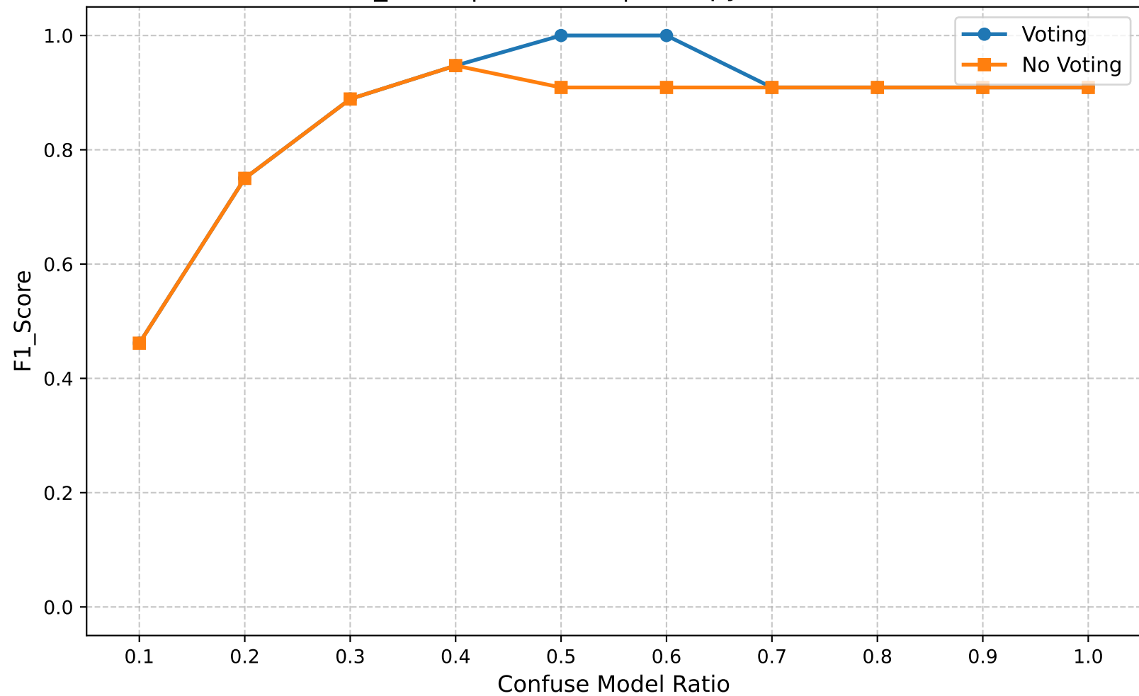
F1_Score | Round 25 | Entropy Ratio 0.45
