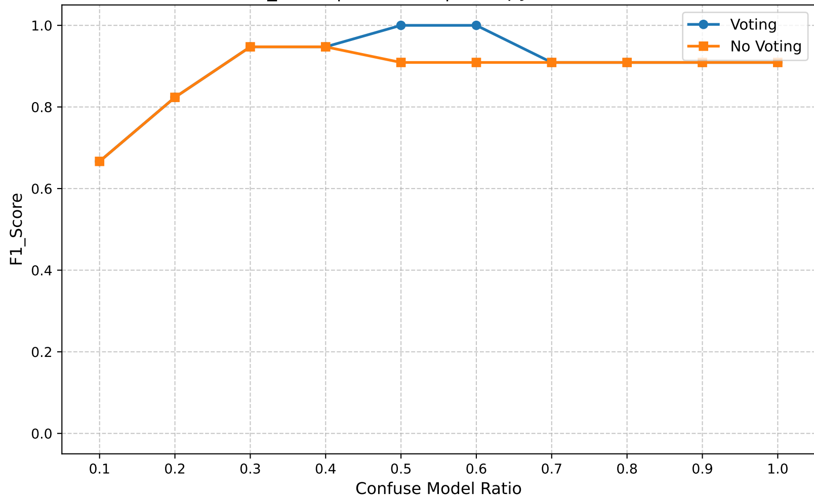
F1_Score | Round 25 | Entropy Ratio 0.50
