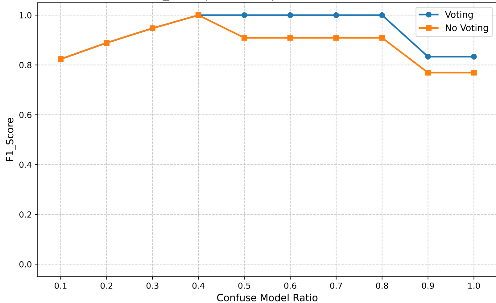
F1_Score | Round 25 | Entropy Ratio 0.60
