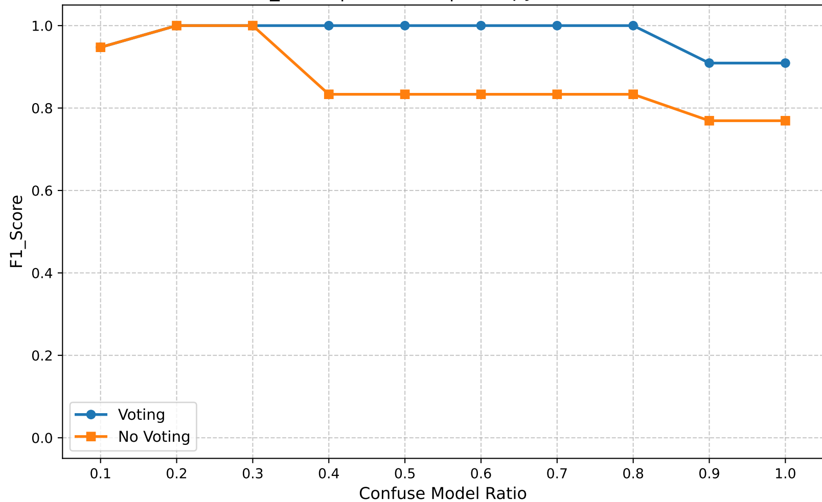
F1_Score | Round 25 | Entropy Ratio 0.65
