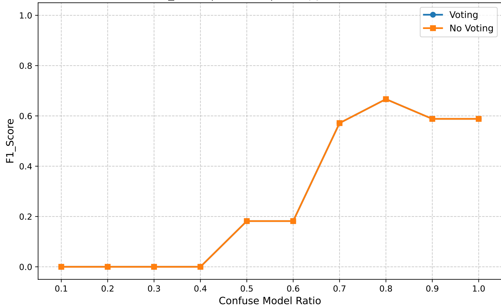
F1_Score | Round 5 | Entropy Ratio 0.10
