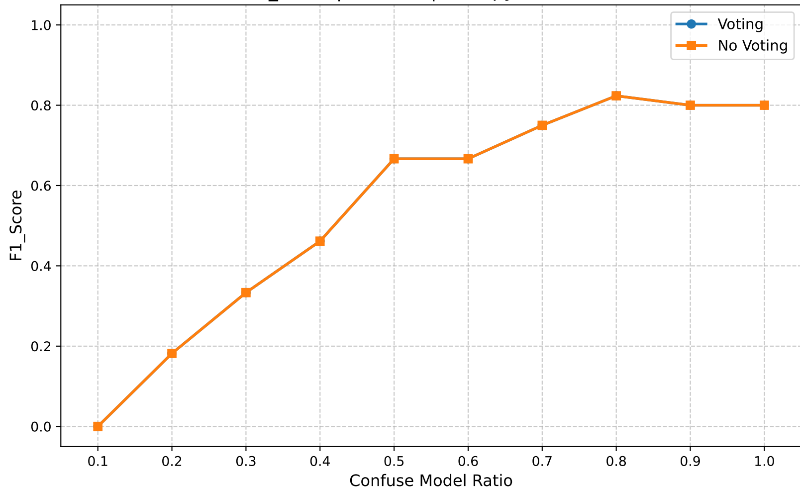
F1_Score | Round 5 | Entropy Ratio 0.20
