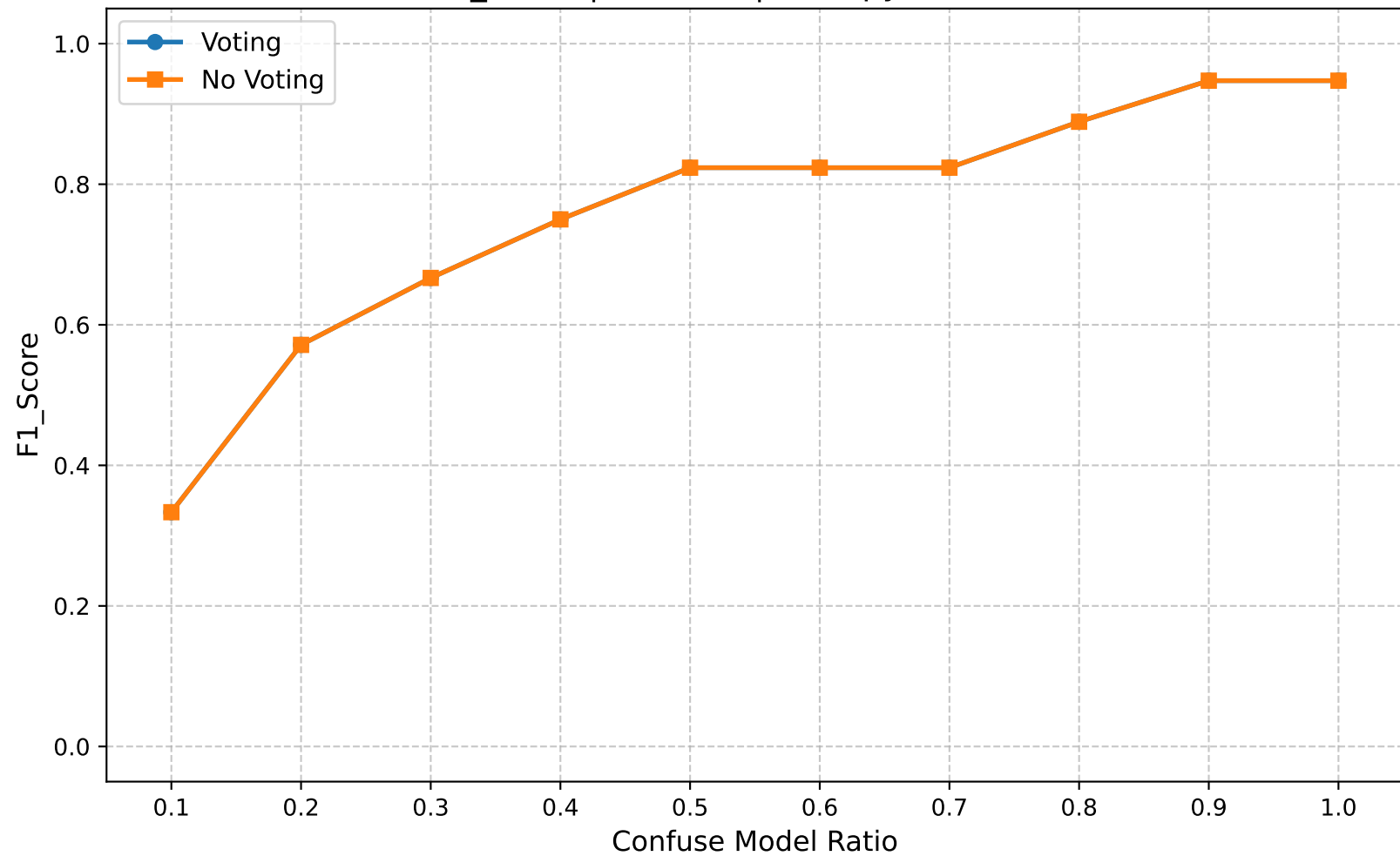
F1_Score | Round 5 | Entropy Ratio 0.30
