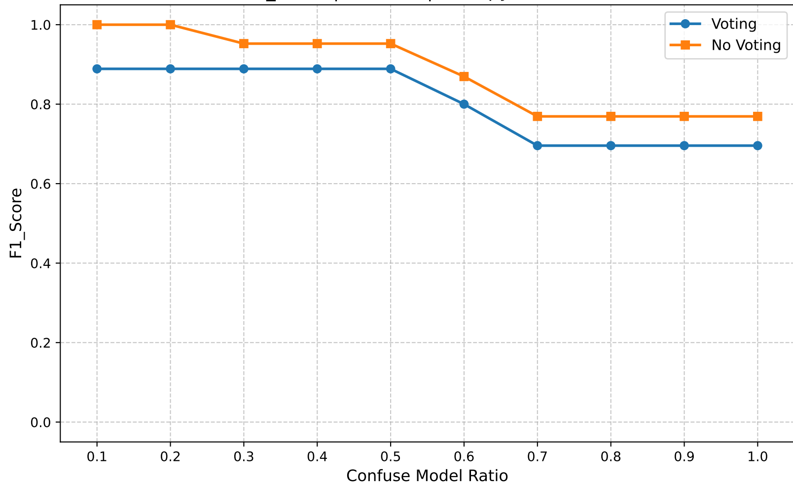
F1_Score | Round 5 | Entropy Ratio 0.80
