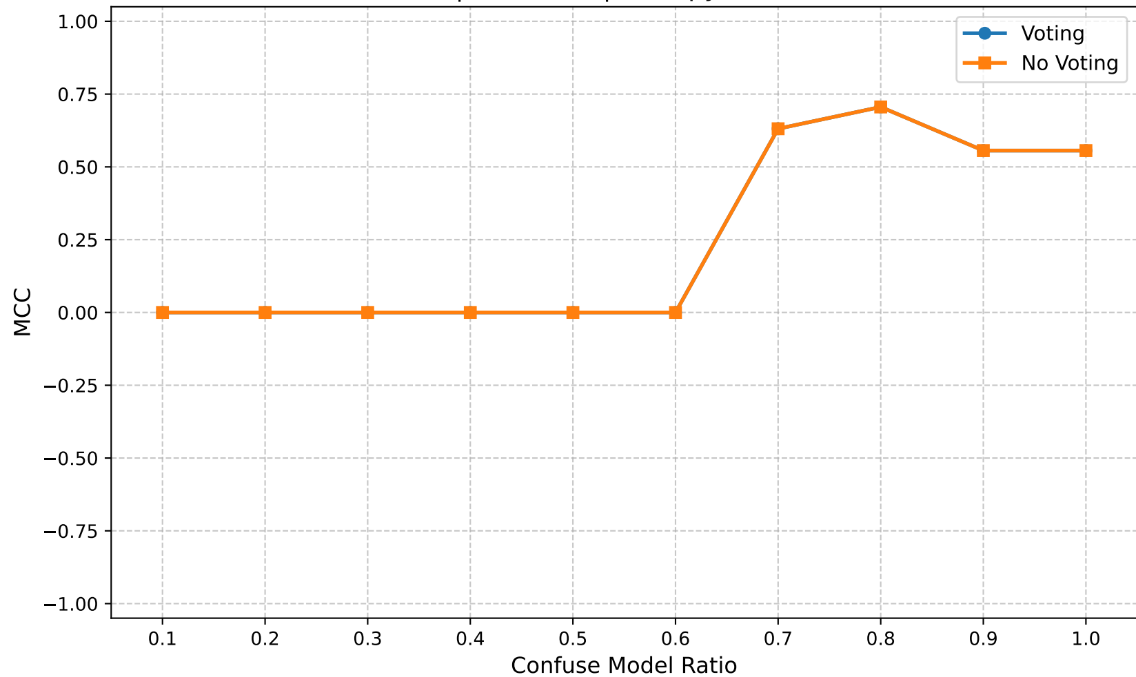
MCC | Round 10 | Entropy Ratio 0.10
