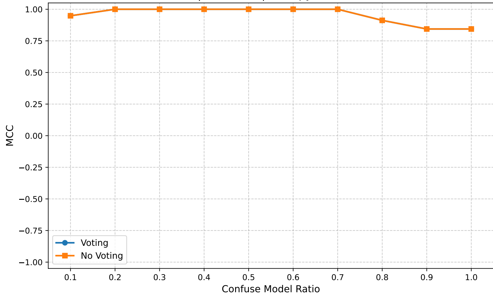
MCC | Round 10 | Entropy Ratio 0.65
