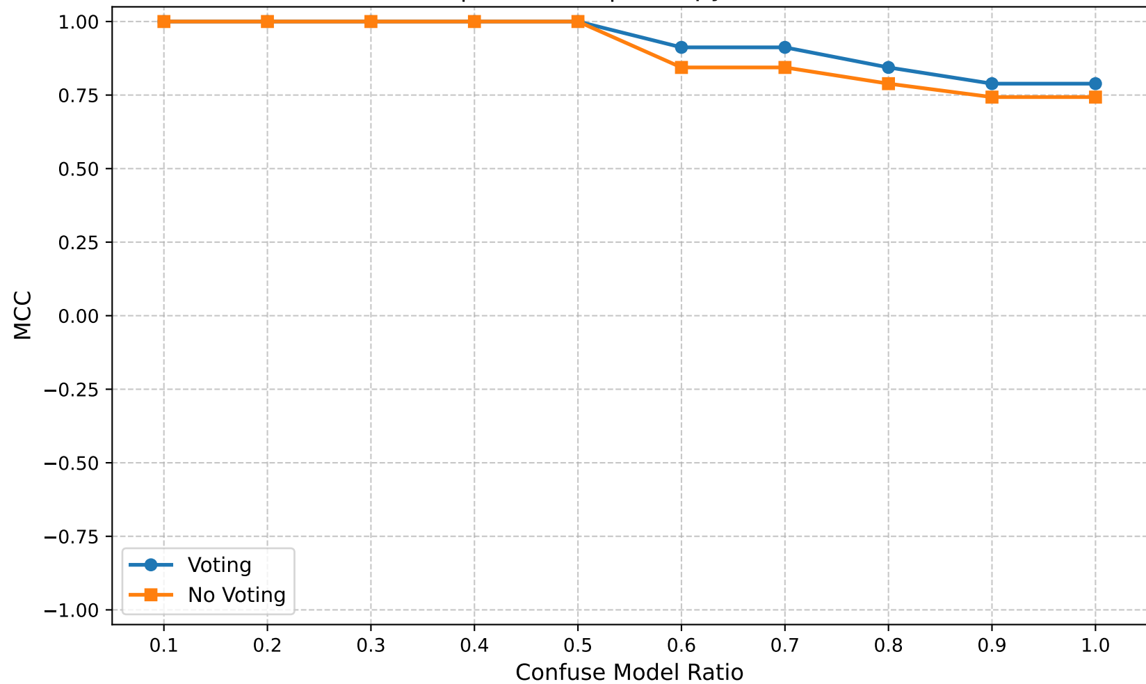
MCC | Round 10 | Entropy Ratio 0.75
