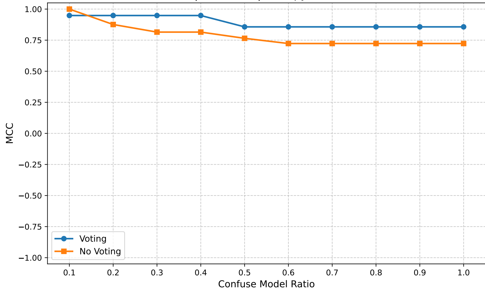
MCC | Round 15 | Entropy Ratio 0.85
