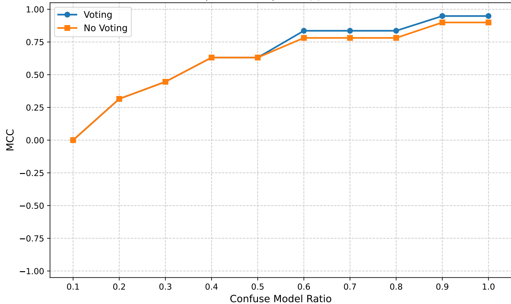
MCC | Round 20 | Entropy Ratio 0.30
