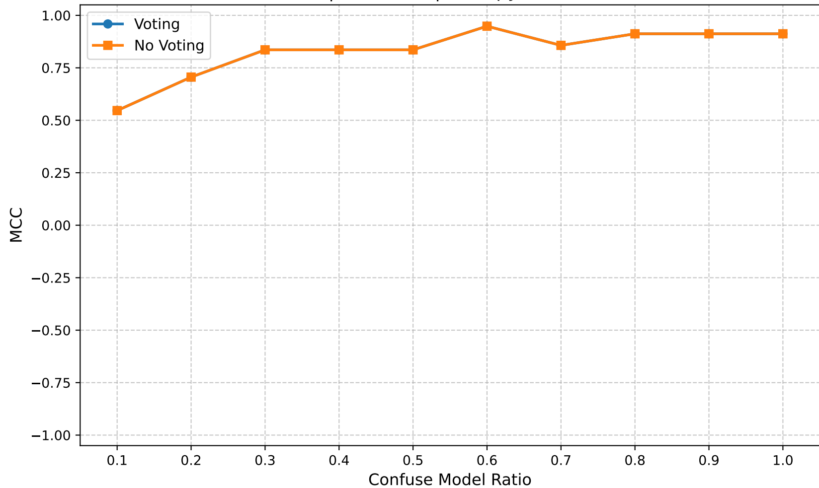
MCC | Round 20 | Entropy Ratio 0.40
