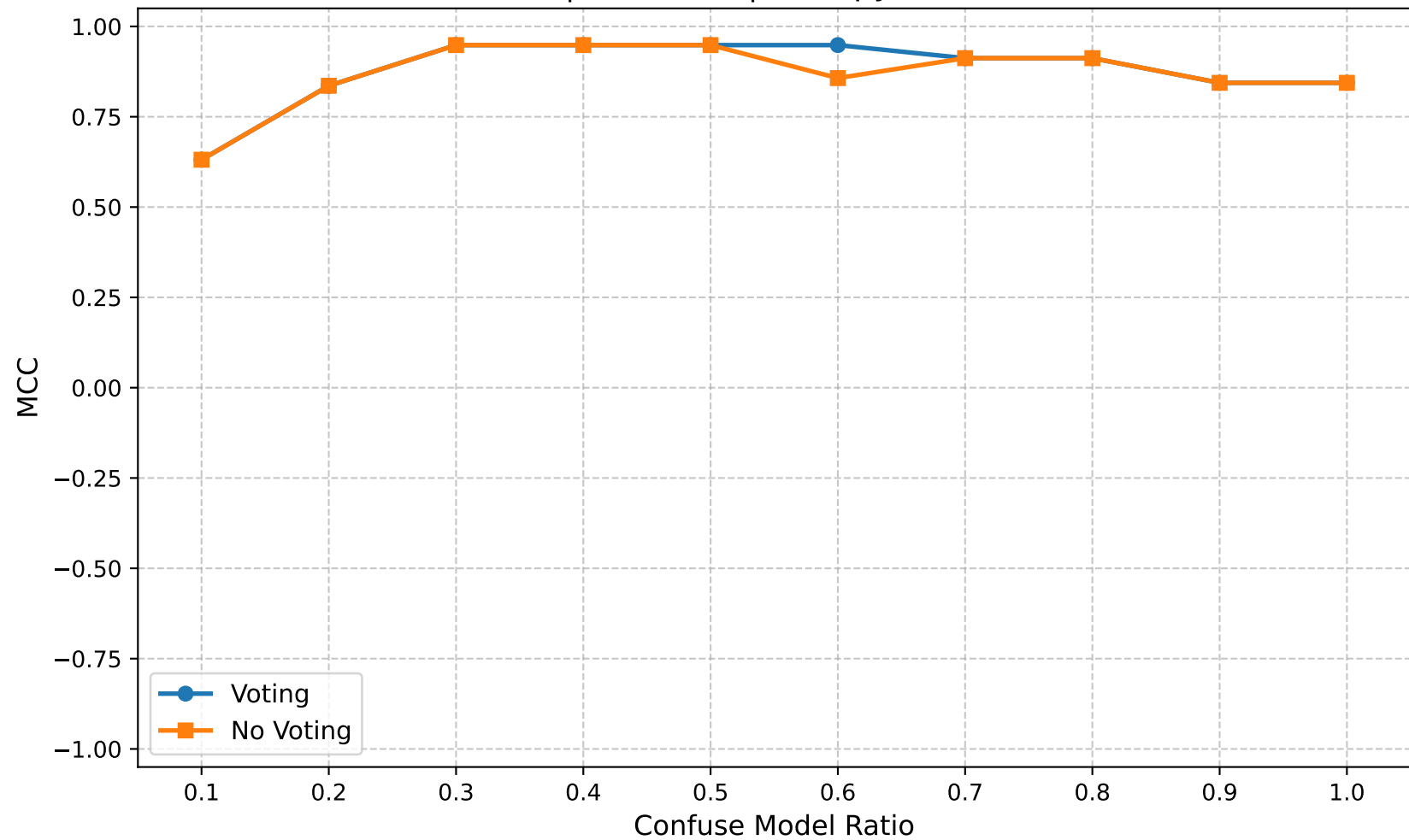
MCC | Round 20 | Entropy Ratio 0.50
