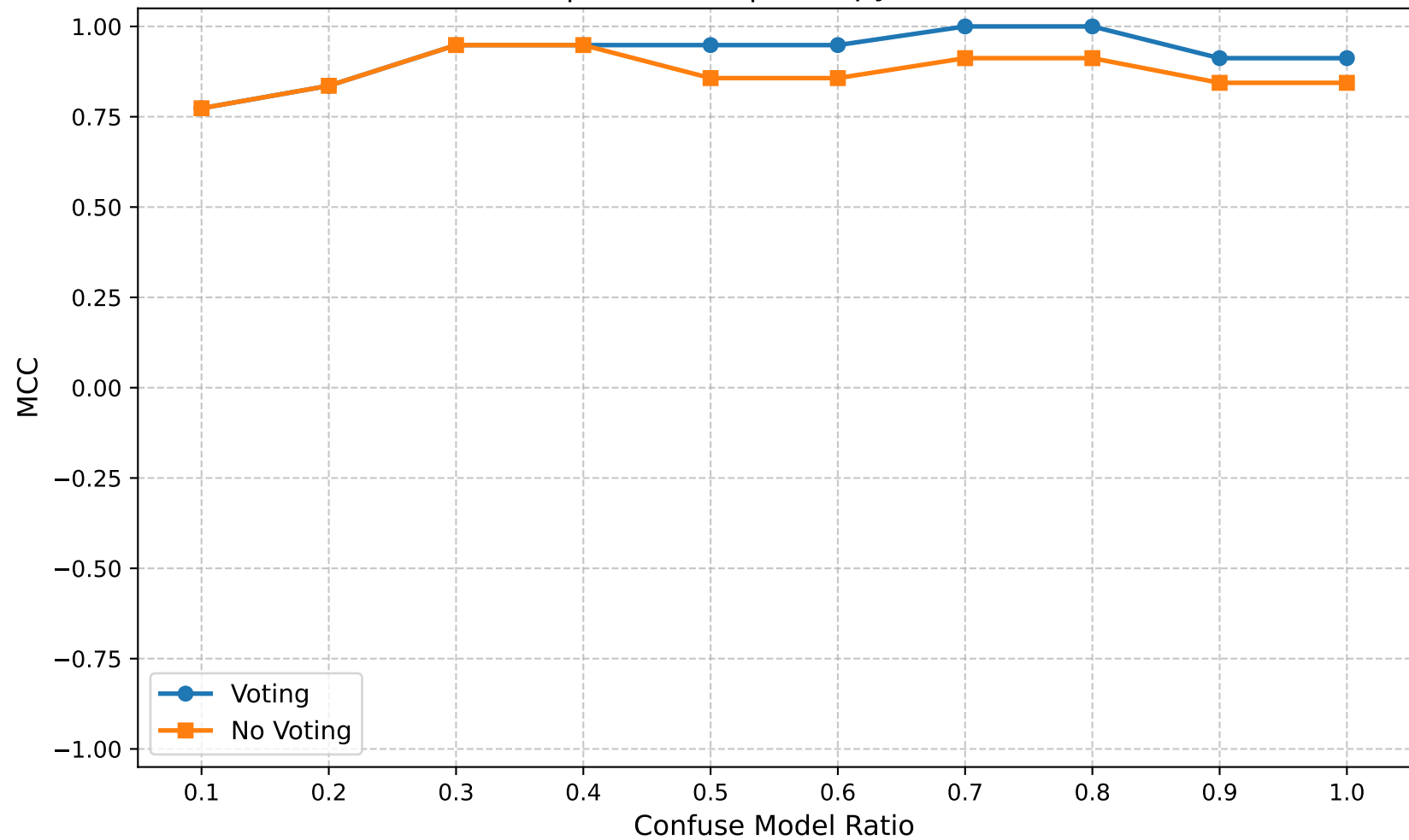
MCC | Round 20 | Entropy Ratio 0.55
