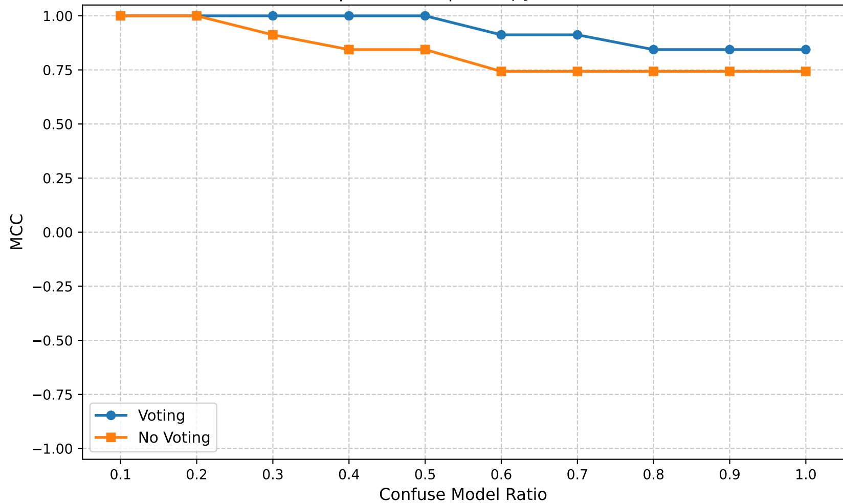
MCC | Round 20 | Entropy Ratio 0.80
