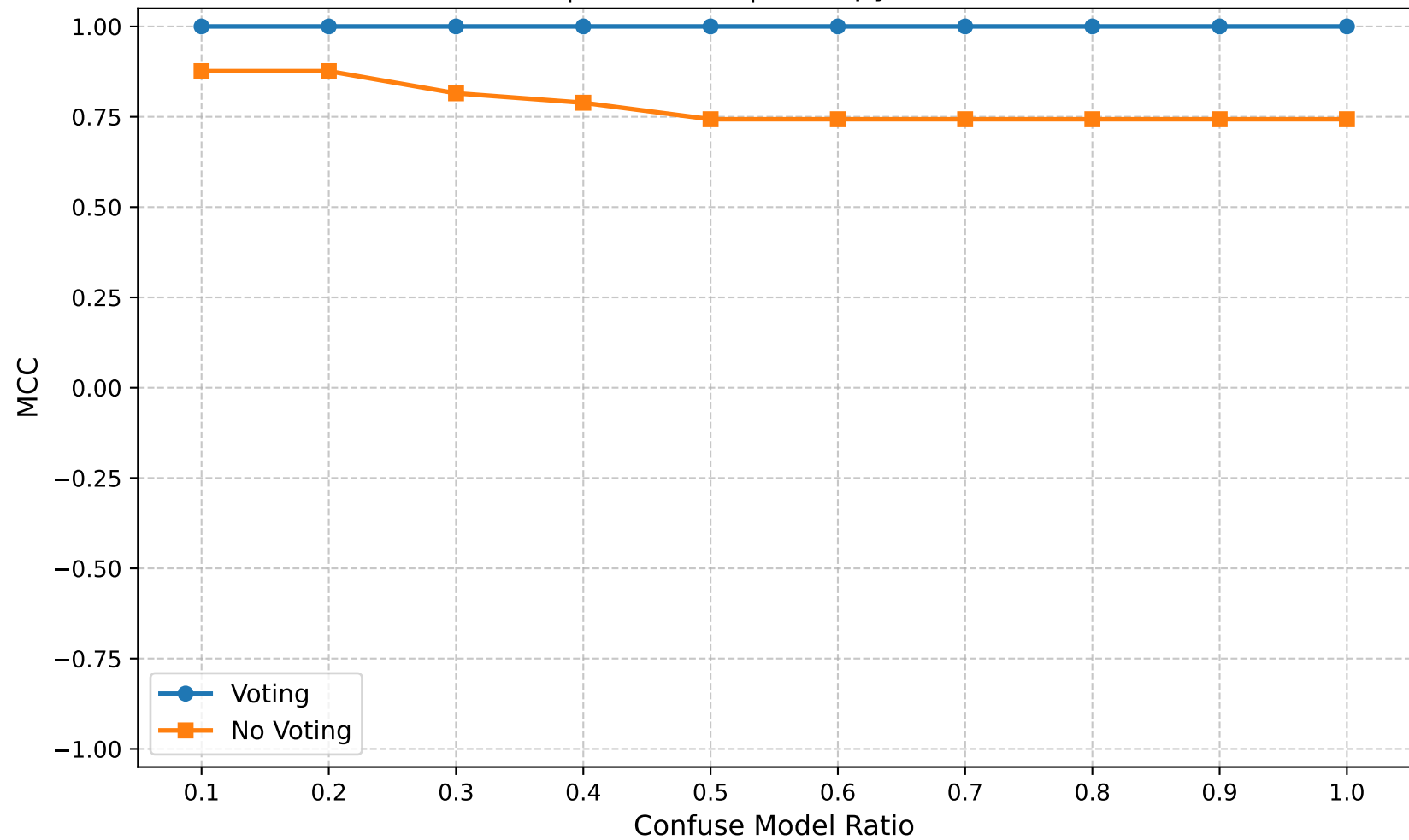
MCC | Round 20 | Entropy Ratio 0.90
