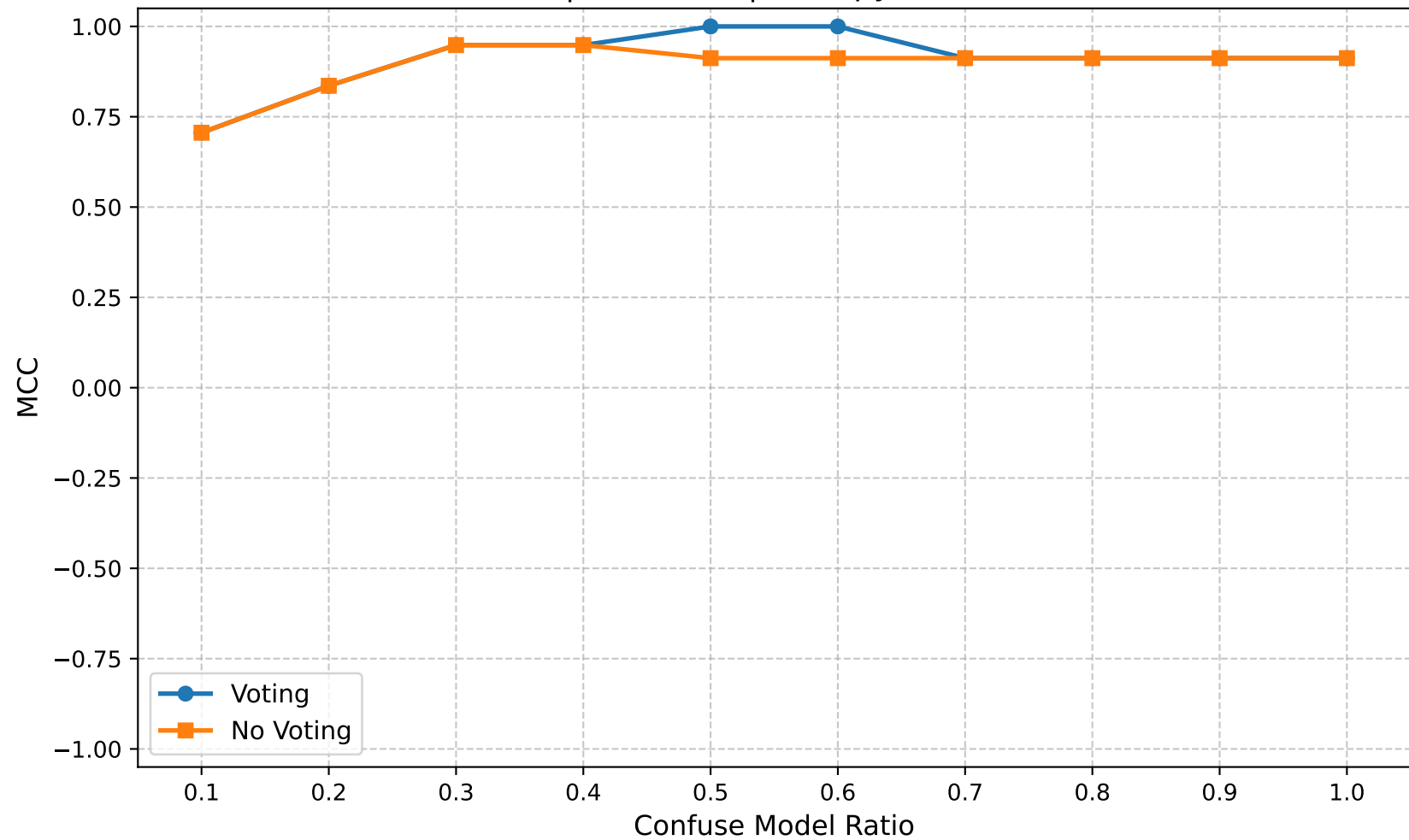
MCC | Round 25 | Entropy Ratio 0.50
