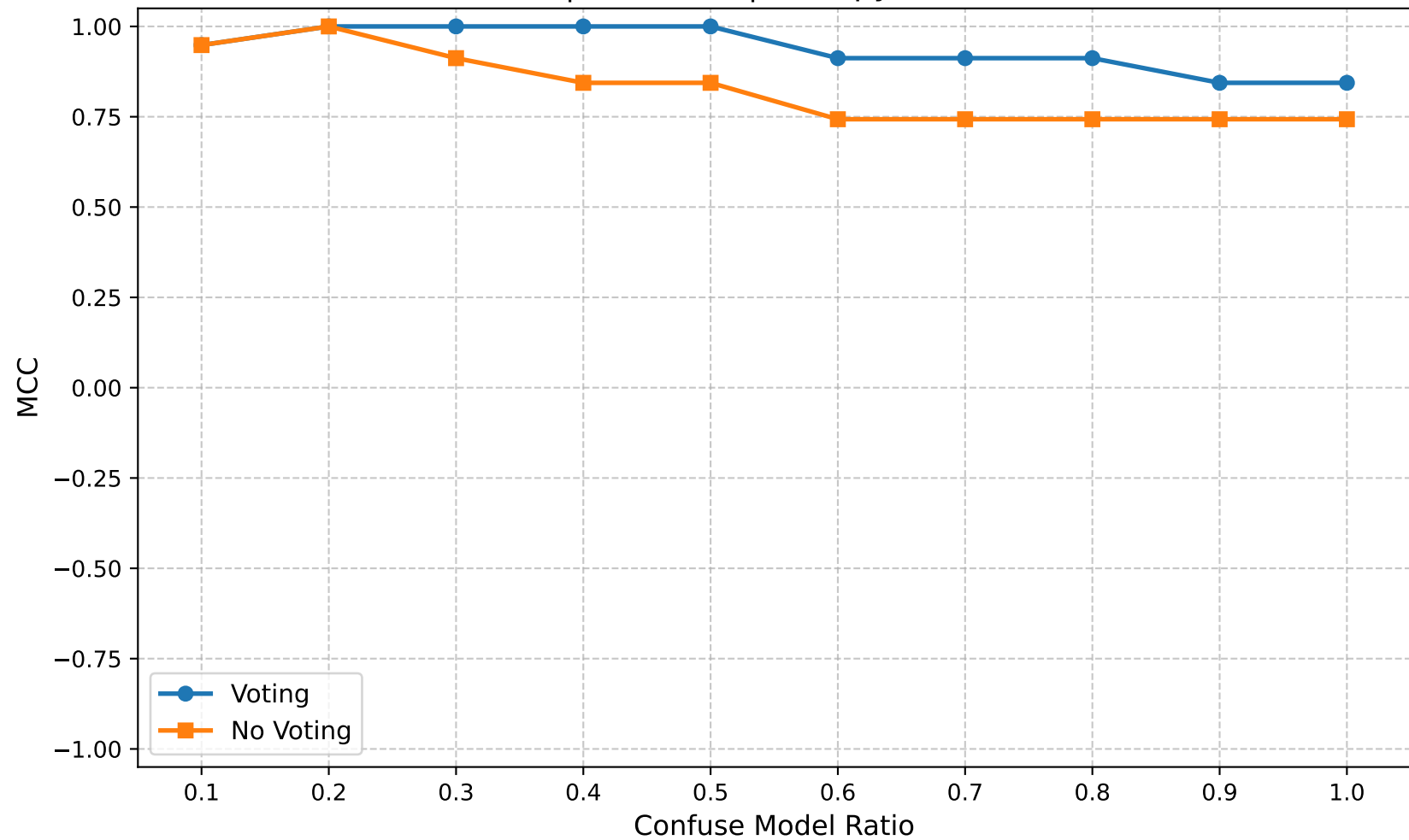
MCC | Round 25 | Entropy Ratio 0.75
