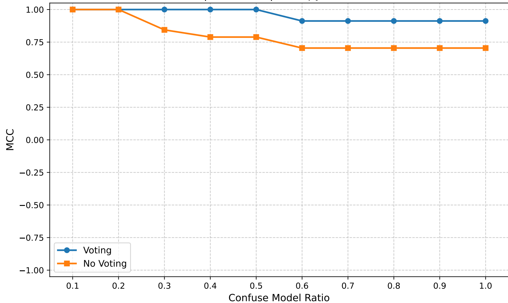
MCC | Round 25 | Entropy Ratio 0.80
