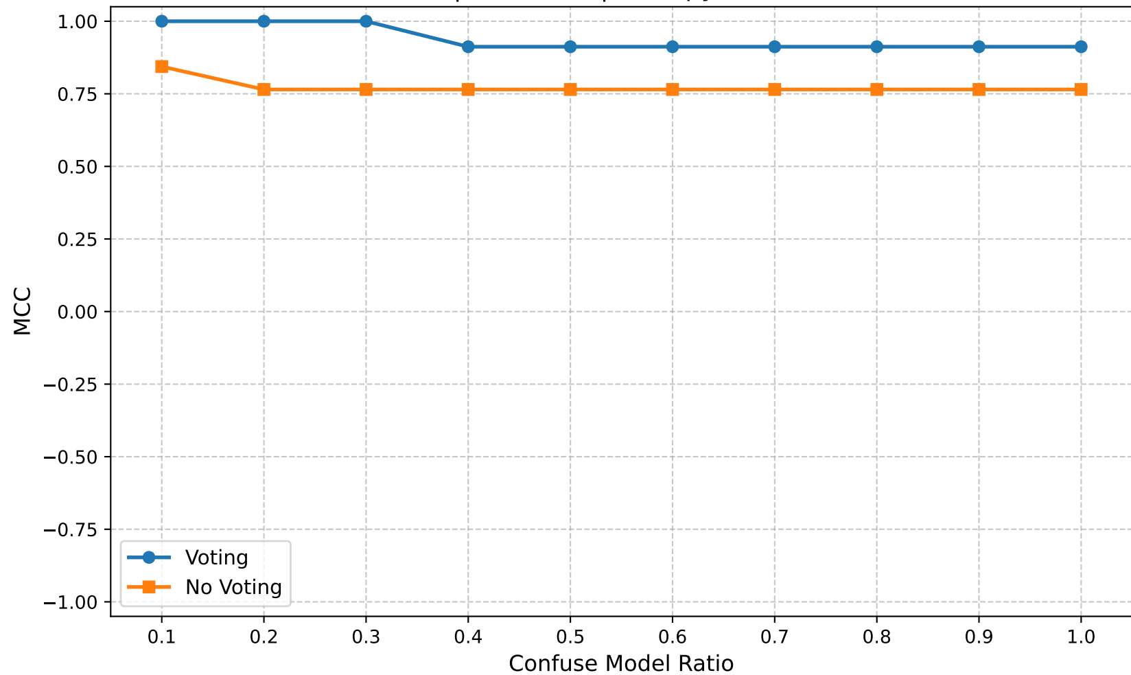
MCC | Round 25 | Entropy Ratio 0.95
