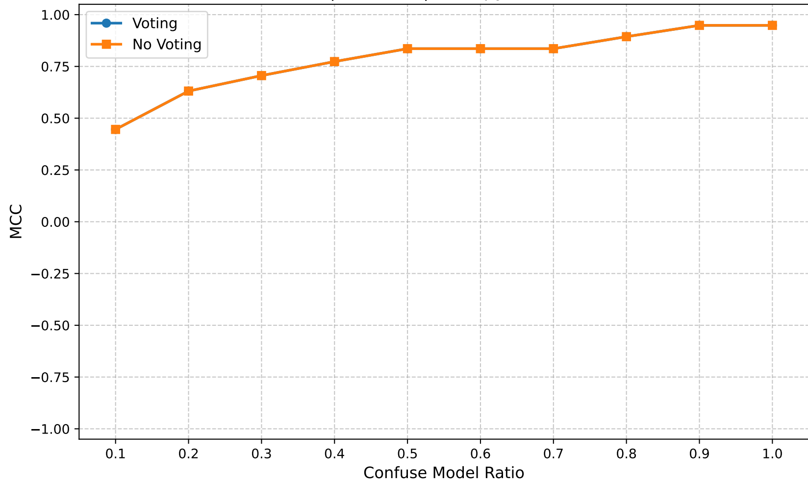
MCC | Round 5 | Entropy Ratio 0.30
