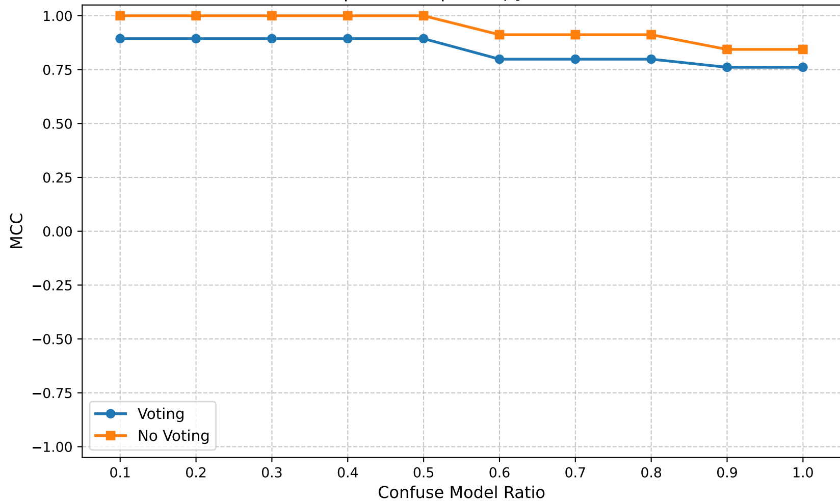
MCC | Round 5 | Entropy Ratio 0.70
