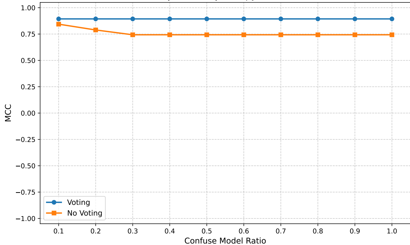
MCC | Round 5 | Entropy Ratio 0.95
